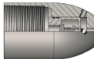
FloCheck Passive Check-Valve Guide Shoe
