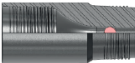
FloCheck Passive Ball Seat Sub
